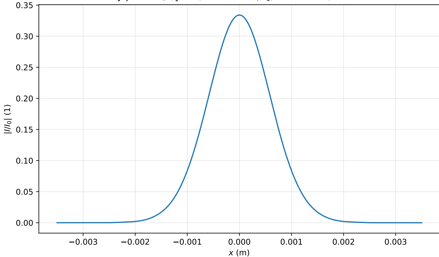
Intensity profile I(x, y = 0, z = 3.264m)/I_0 , P_{in}=0.2P_{cr} , artificial time
